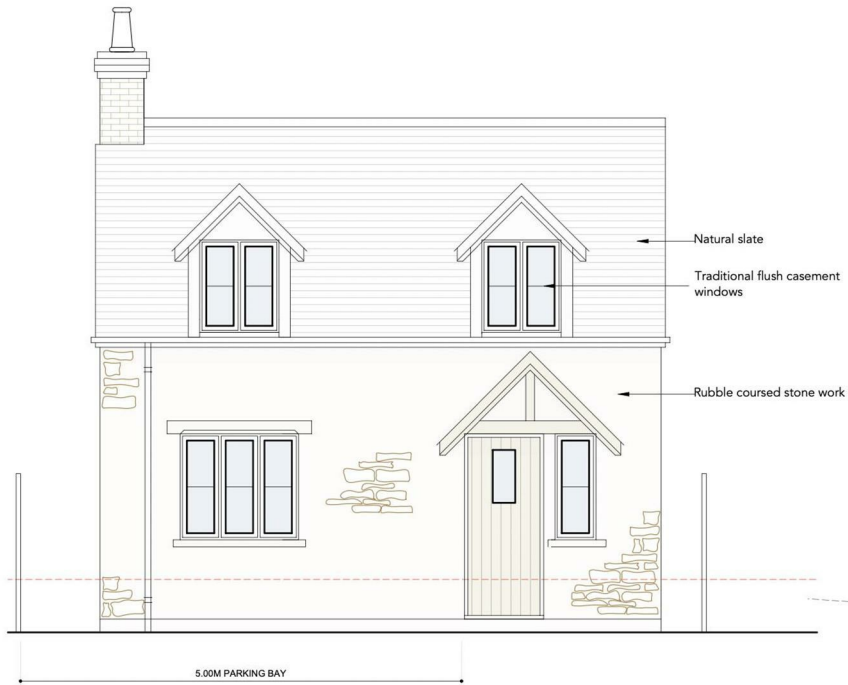
SOUTH ELEVATION 1-50
